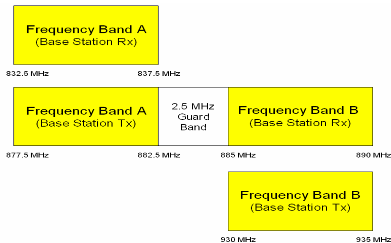
Figure 2: Guard band between Frequency Bands A and B
